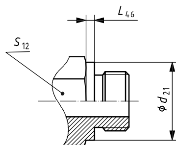
Figure A.6 — Reduced ISO 11926-3 stud end
